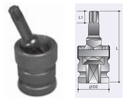
Universal Internal Torx Drivers
