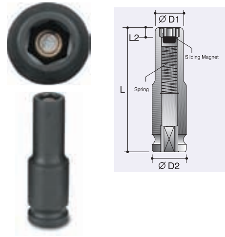
6-Point Sockets - Deep
