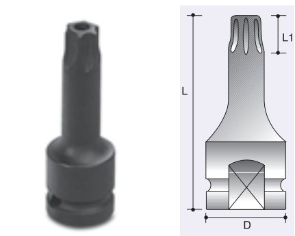
Internal Torx Drivers - With Tamper Resistant
