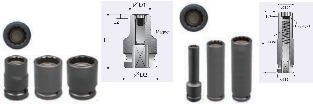
12-Point Sockets
