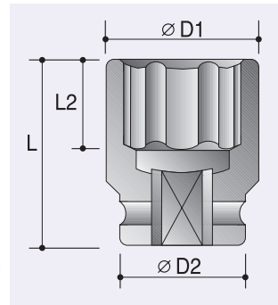
4-Point Sockets
