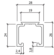
CALHA DE 5mt/4mt/2mt/ RAILING 5mt/4mt/2mt/
