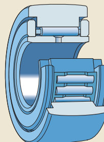
Support roller with flange rings
